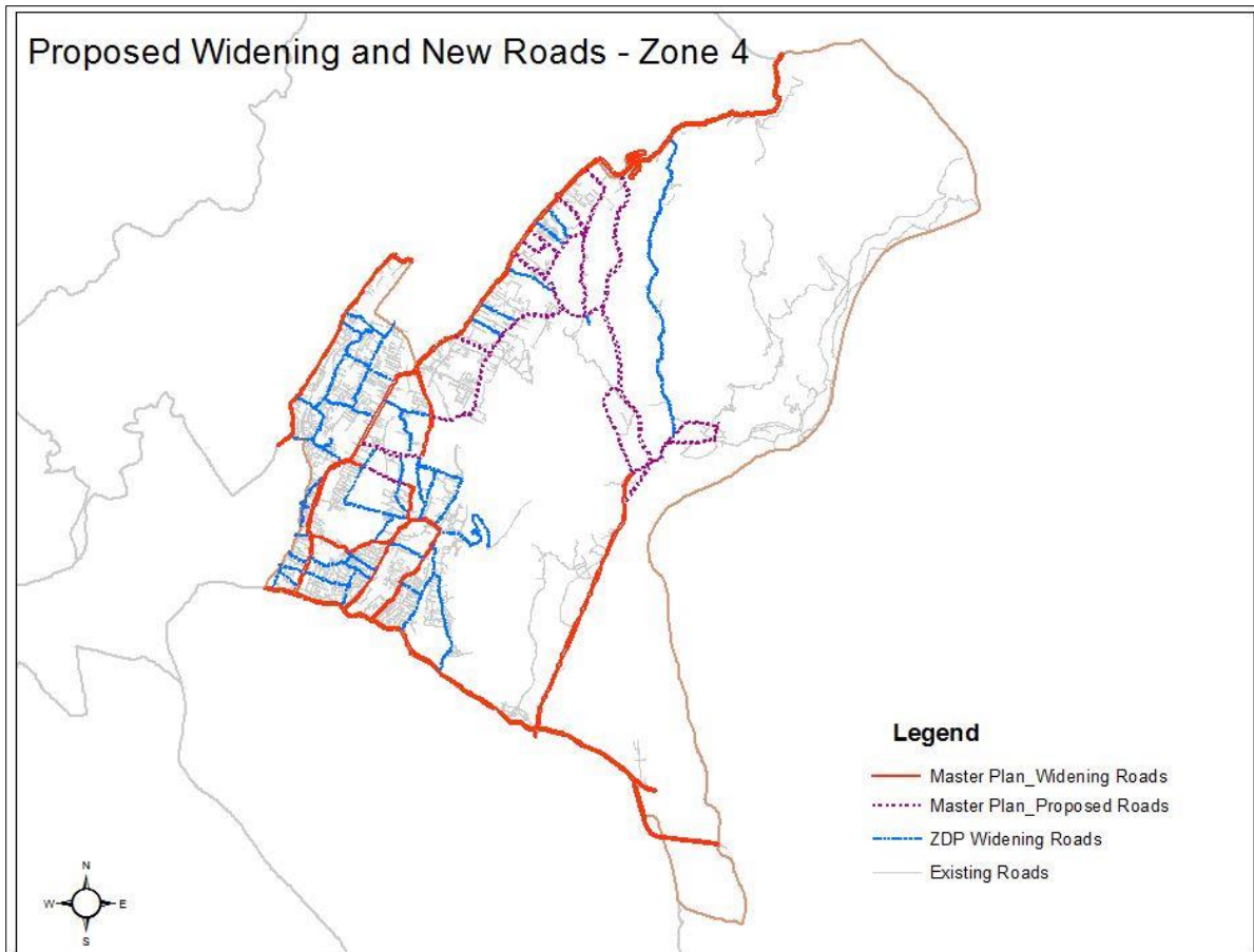
Figure 9 : Map showing the road widening proposals
